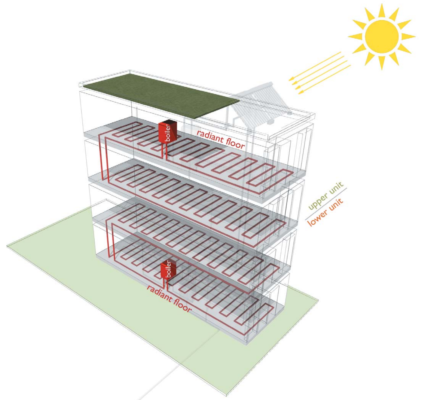
heating system: radiant floor heating
