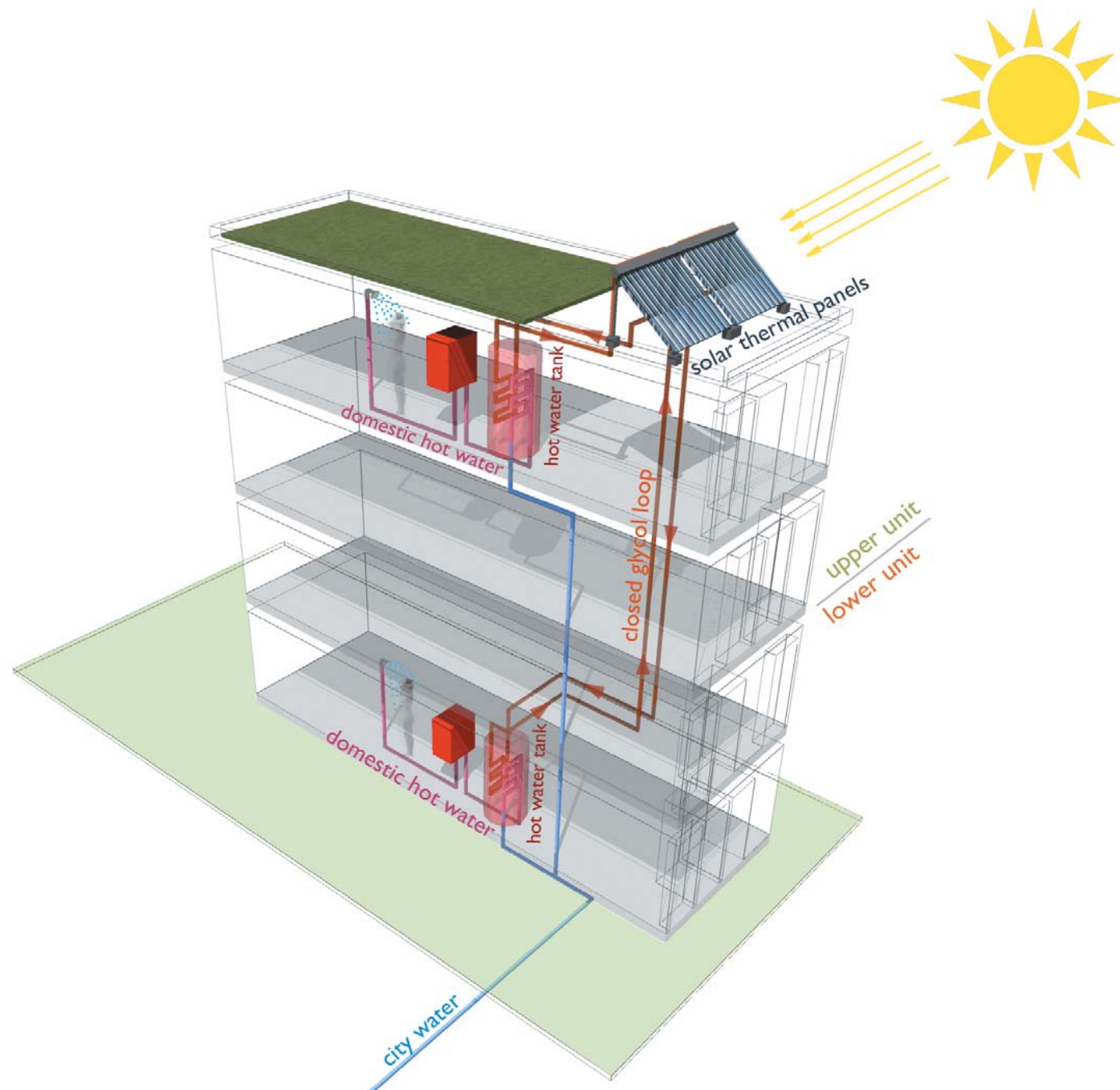
domestic hot water: flat plate solar thermal panels provides 100% of hot water
